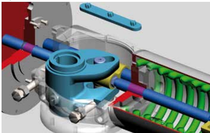
Symetric yoke mechanism Spring to close
