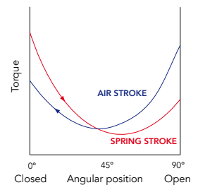
Symetric yoke mechanism Spring to open
