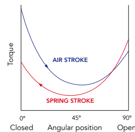
Symetric yoke mechanism Spring to close
