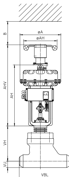
Series 190 globe style actuator type 812
