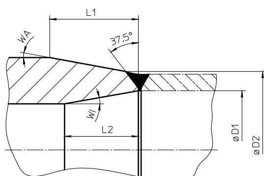
Butt-weld ends acc. to ASME B16.25
