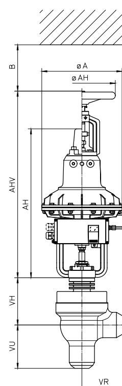
Series 190 angle style actuator type 811
