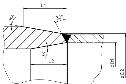
Butt-weld ends acc. to DIN EN 12627
